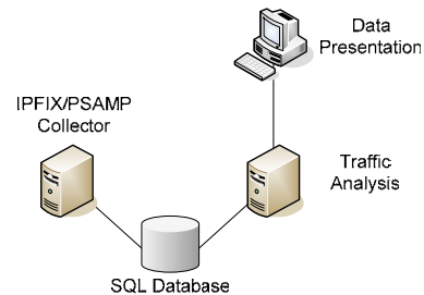
Figure 3. NASTY architecture
