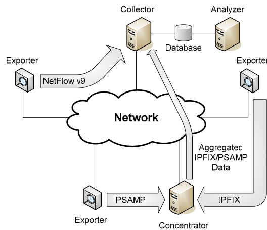
Figure 1. HISTORY architecture
