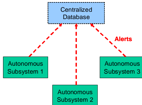
Fig 1. Distributed detection system with autonomous subsystems
